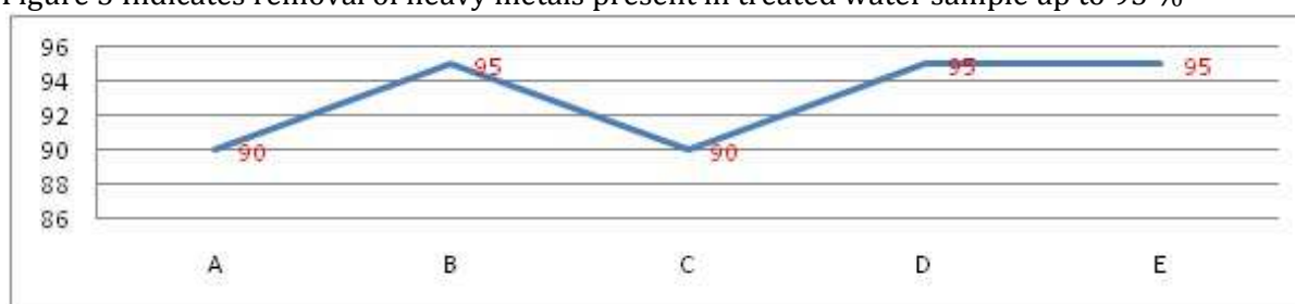
Figure 3 Indicates removal of heavy metals present in treated water sample up to 95 %
